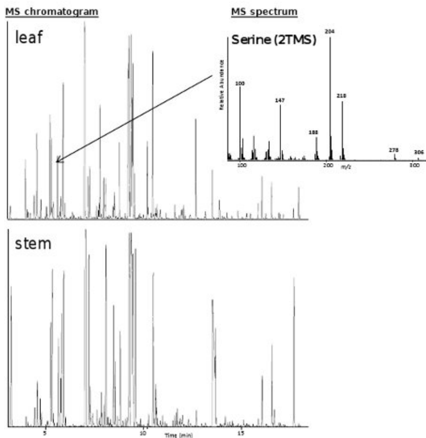
Figure 2. MS chromatogram and spectrum of N. glauca tissue extracts. Total ion MS chromatogram (TIC) of leaf and stem extracts measured by GC-MS is presented (70-600 m/z ). GC-MS analysis was performed as described previously in 15 . Detected peaks were annotated using the mass spectral tags library. MS spectrum of serine (2TMS) is shown as an example. MS chromatogram: X axis and Y axis indicate retention time (min) and the intensity (abundance) of the signal, MS spectrum: X axis and Y axis indicate the M/Z ratios and the intensity (abundance) of the signal, respectively. Click here to view larger image.
